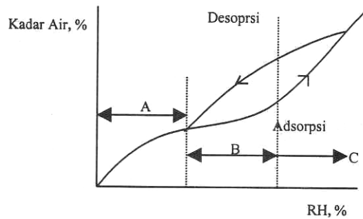
Gbr. 2. Isoterm Sorpsi Lembab
